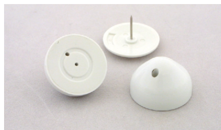
R30 No.T160 Frequency: 8.2MHz Dimension: Ø30mmx18mm Color: Gray or Customized Lock: Standard/Super Packing: 40.5x30.5x20cm, 1000pcs/ctn, 8.76kgs/ctn
