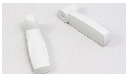
Flat Pencil Tag No.T069 Frequency: 8.2MHz/58KHz Dimension: 53mmx15mm Color: Gray or Customized Lock: Standard/Super/Super S Packing: 34x25x19cm, 1000pcs/ctn, 9.45kgs/ctn(8.2MHz), 10.0kgs/ctn(58KHz)
