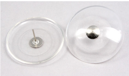
Pin No.P16 Length: 16mm/19mm/21mm Remark: Groove/Smooth Color: White/Black/Beige/Gray/Transparent Head diameter: Ø51mm Packing: 58.5x39x17.5cm, 10000pcs/ctn, 7.45kgs/ctn
